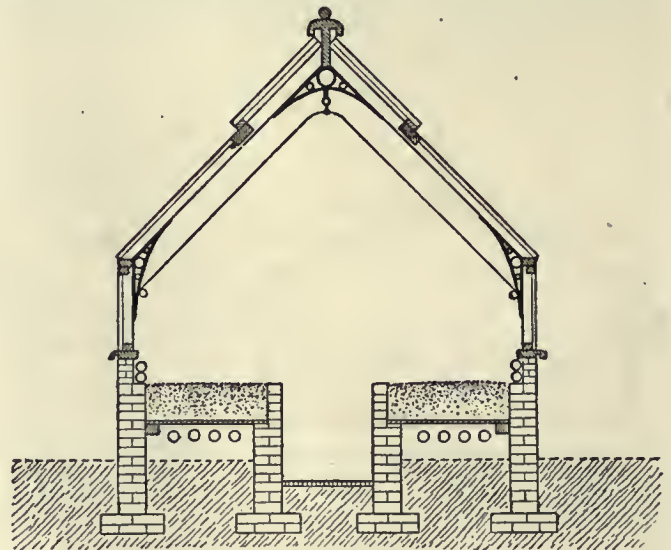
FIG. 9.—Forcing House.
